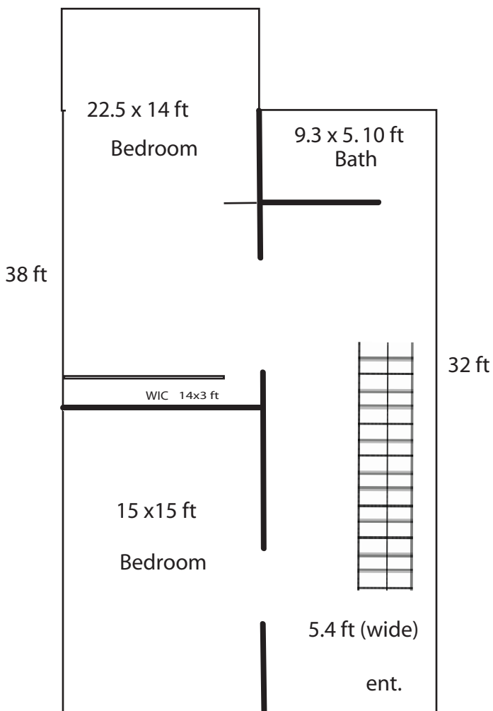
2nd floor 18.9 ft
